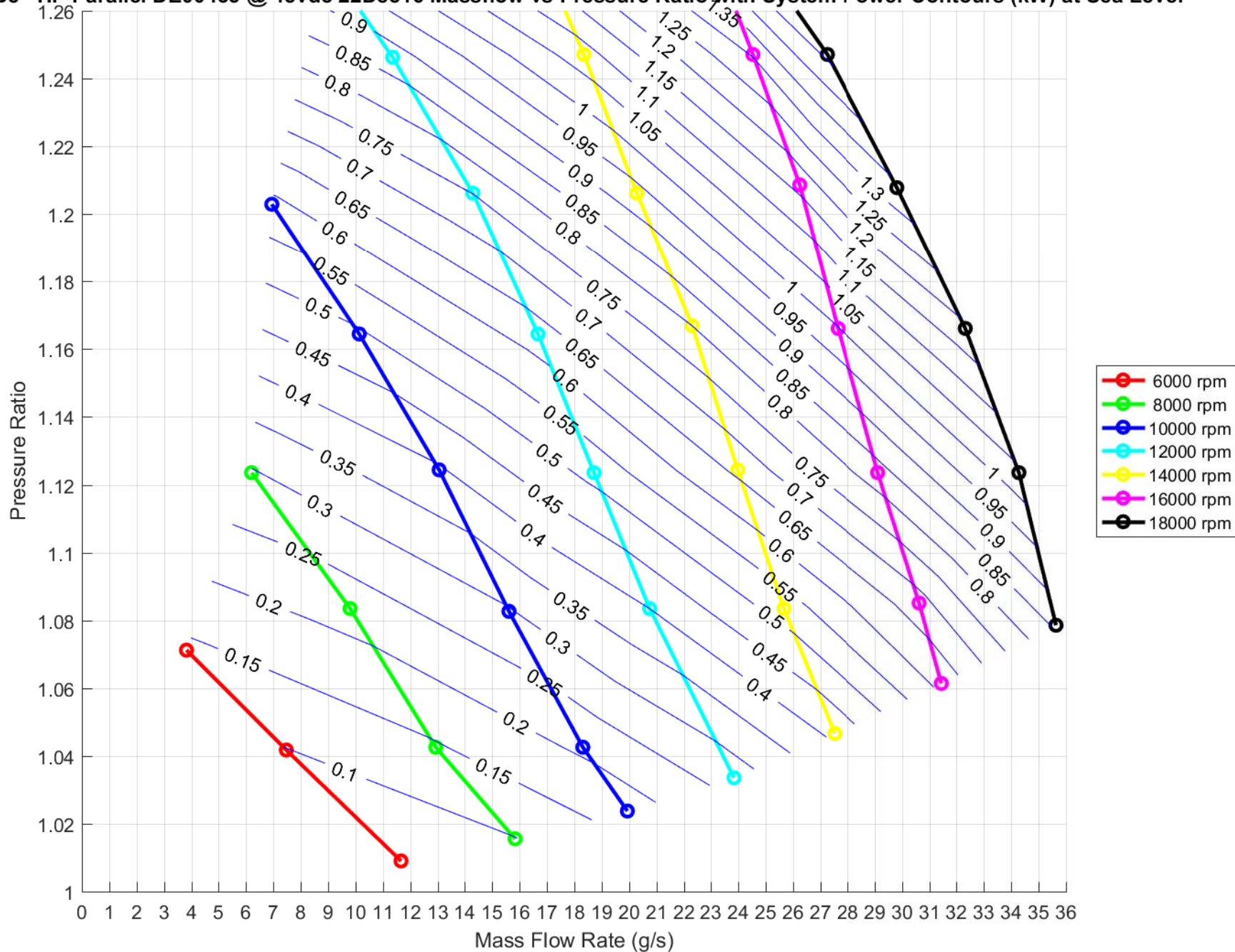
VRB8 2 -HP Parallel DE00433 @ 48vdc 22Dec16 Massflow vs Pressure Ratio with System Power Contours (kW) at Sea Level
