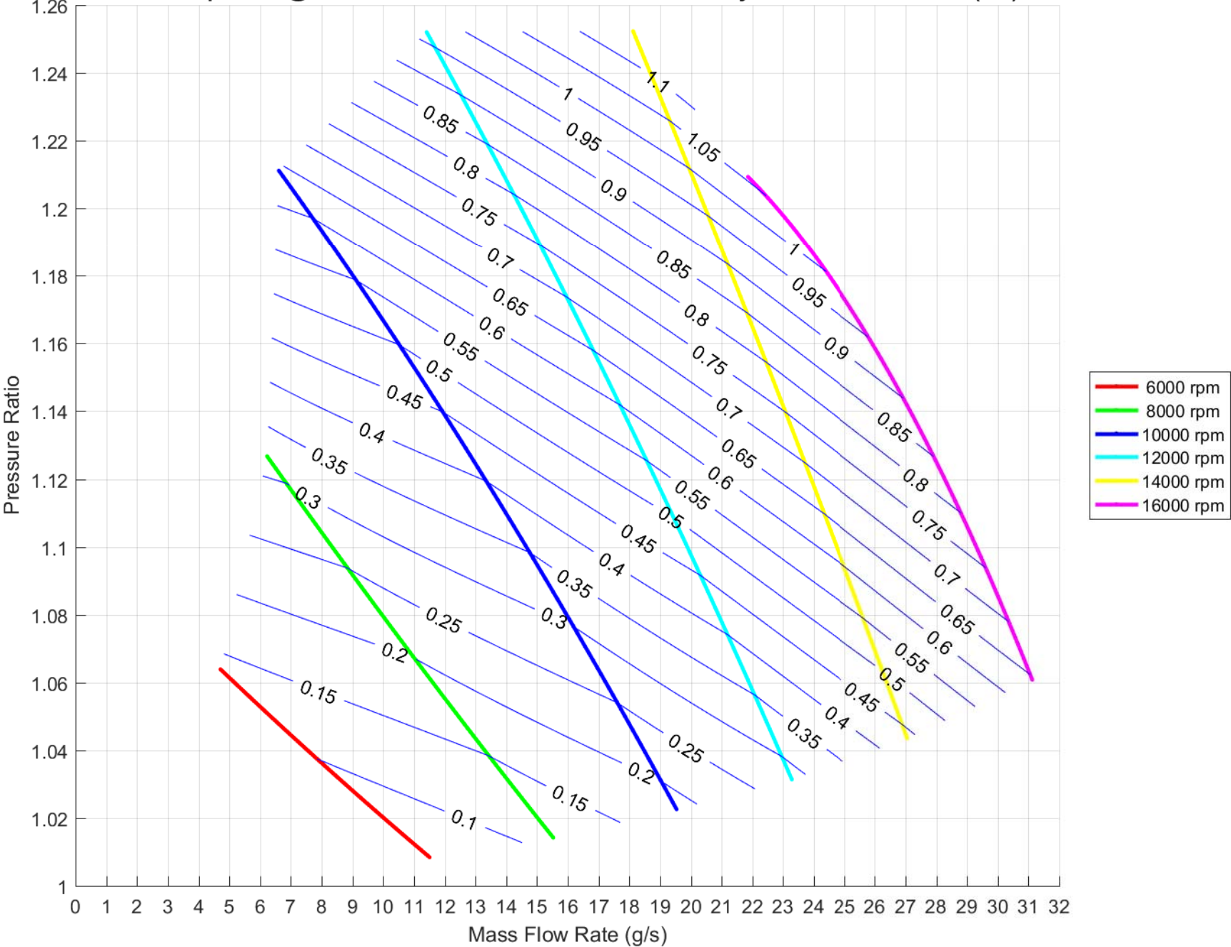
VAIREX VRB8-2-35 in parallel @ 48VDC Massflow vs Pressure Ratio with System Power Contours (kW) at Sea Level
