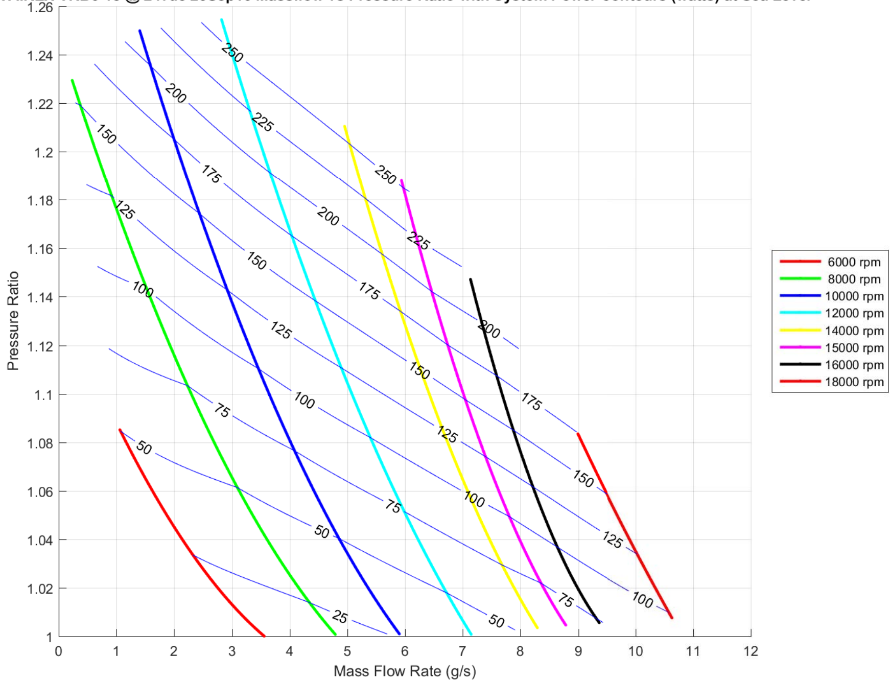
VAIREX VRB6-18 @ 24vdc 23Sep16 Massflow vs Pressure Ratio with System Power Contours (watts) at Sea Level
