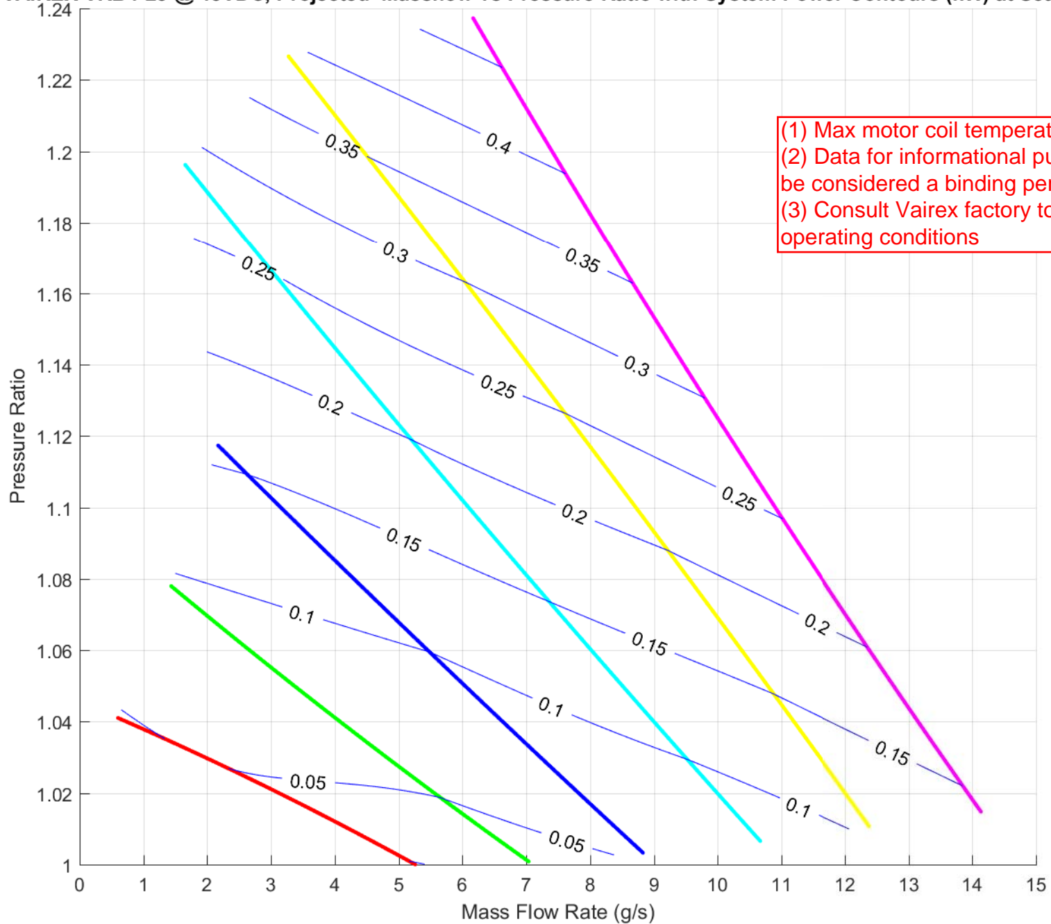
VAIREX VRB4-25 @ 48VDC, Projected Massflow vs Pressure Ratio with System Power Contours (kW) at Sea Level
