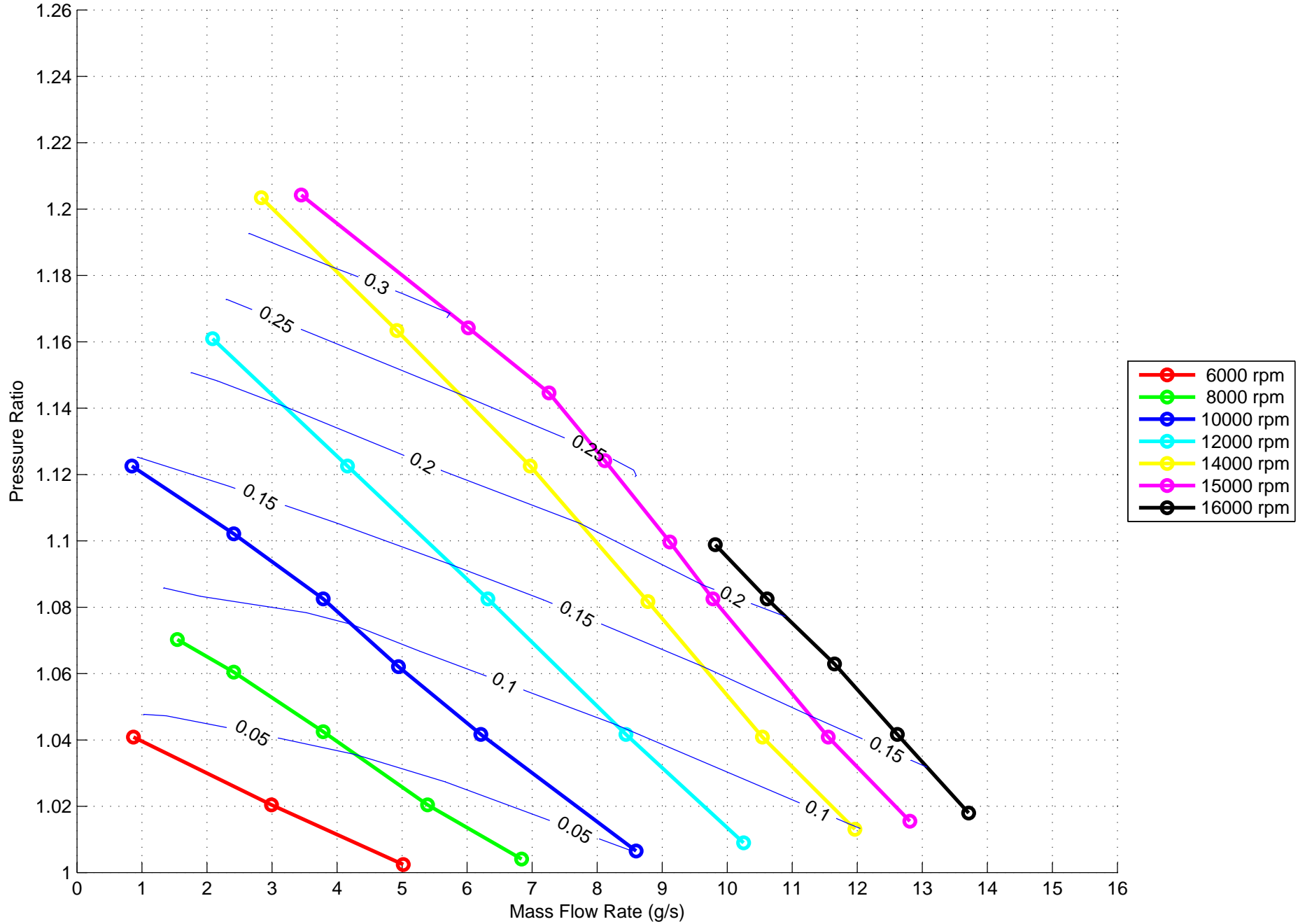
VRB4-25 @ 24vdc 21Nov13 Massflow vs Pressure Ratio with System Power Contours (kW) at Sea Level
