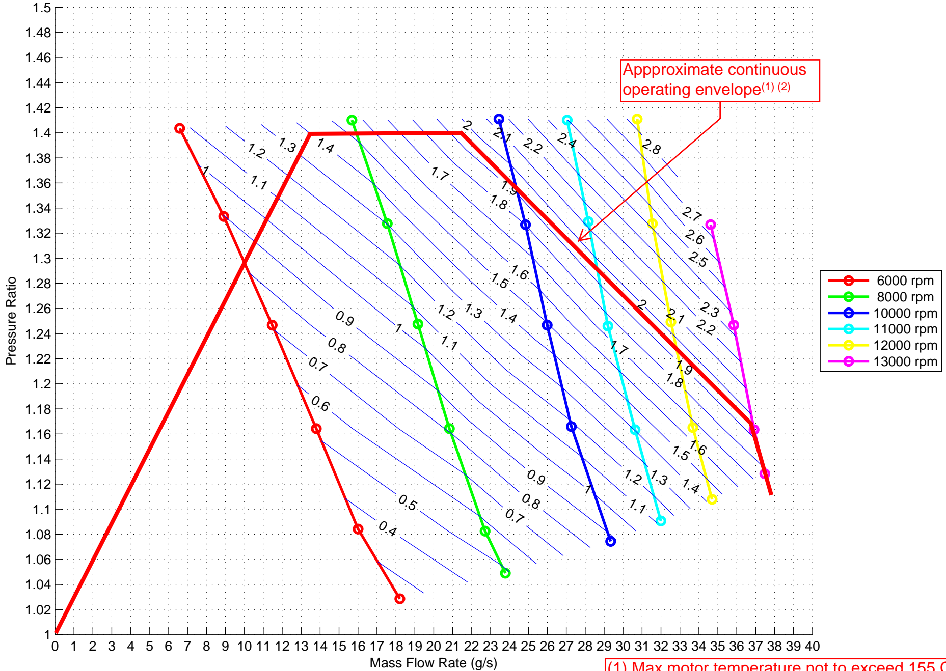
VAIREX VRB32 2 @ 120vdc, Massflow vs Pressure Ratio with System Power Contours (kW) at Sea Level
