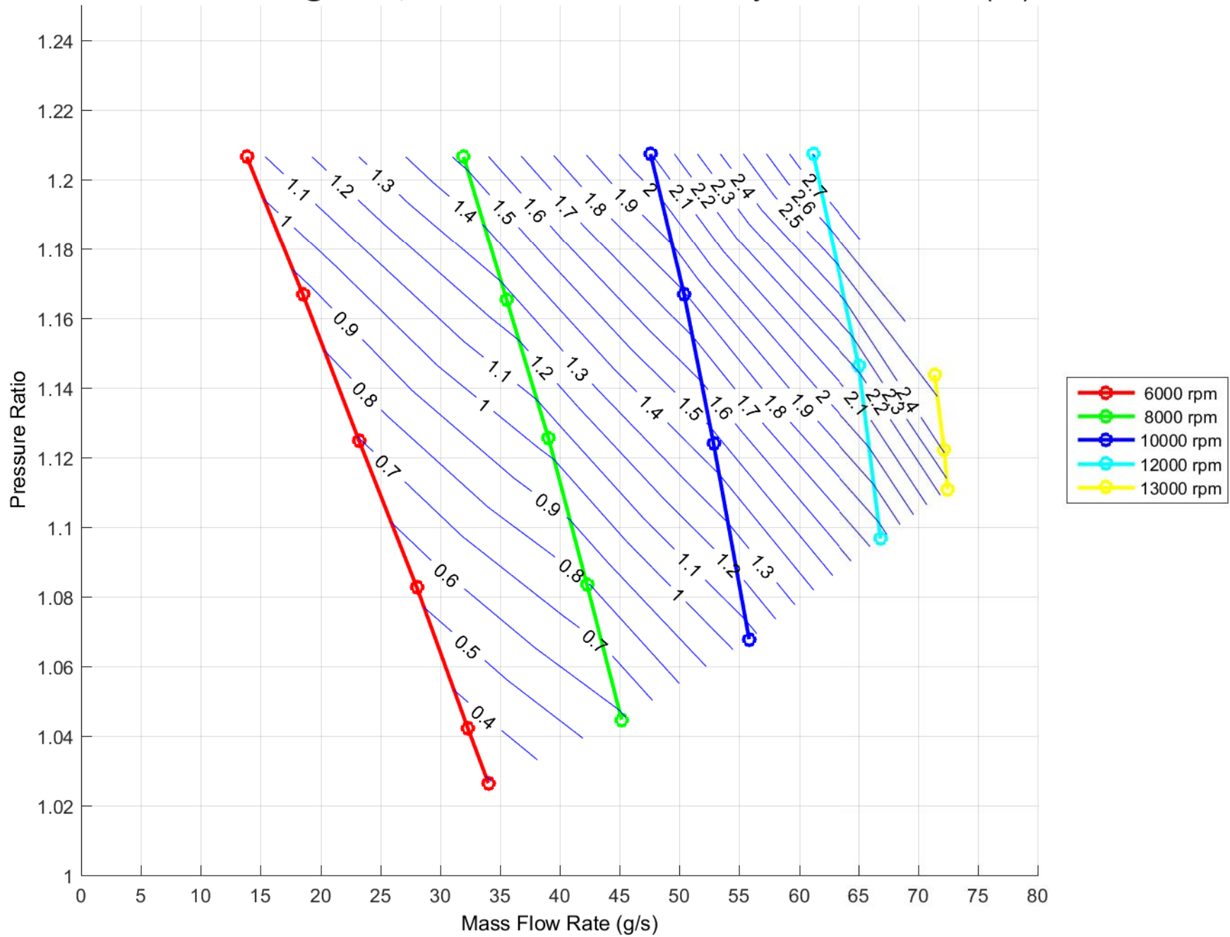
VAIREX VRB64 CG00100 24Mar16 @ 100vdc, Massflow vs Pressure Ratio with System Power Contours (kW) at Sea Level
