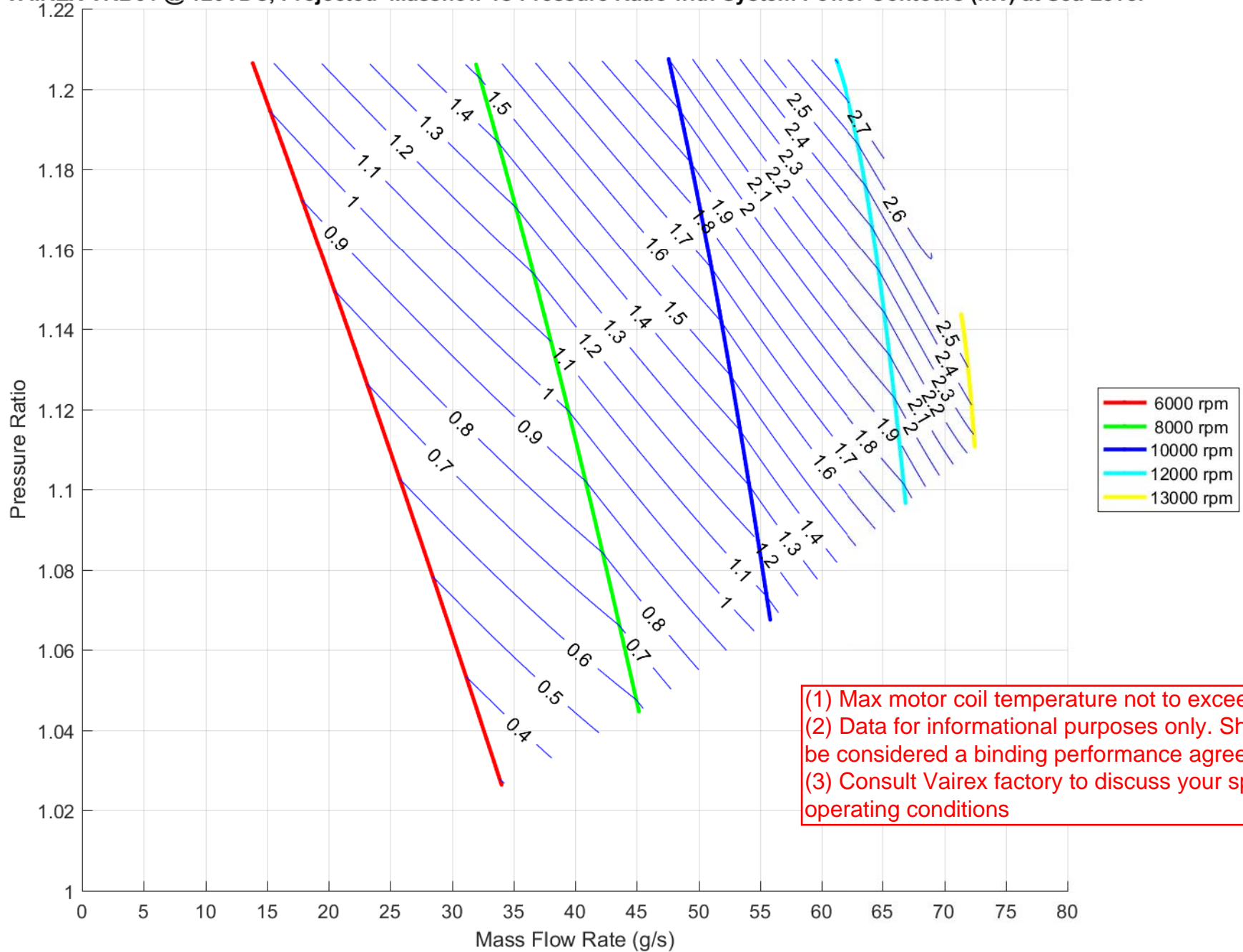
VAIREX VRB64 @ 120VDC, Projected Massflow vs Pressure Ratio with System Power Contours (kW) at Sea Level
